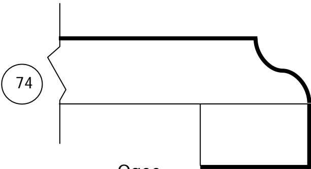
Ogee
